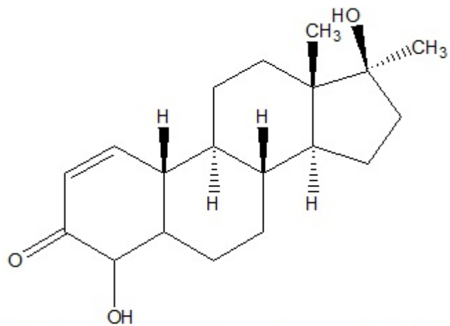
17 \alpha -Methyl-3-oxo-19-norandrostene-4,17-diol
